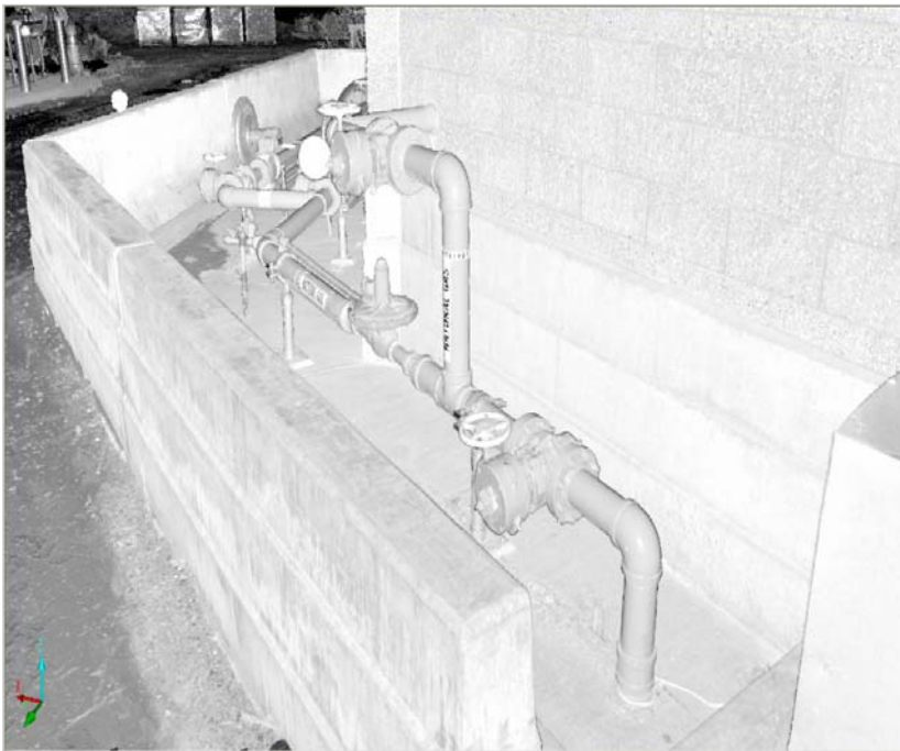
Data from piping on two sides of a building were tied to a common coordinate system to create single, continuous as-built data of the facility exterior.
